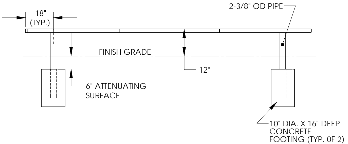
ELEVATION VIEW
